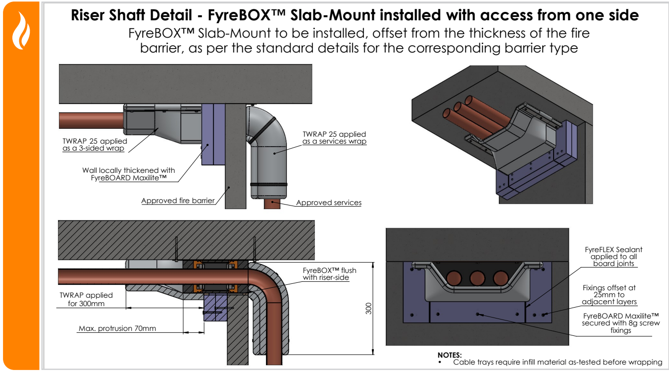
The FyreBOX can be installed offset to the wall using strips of FyreBOARD Maxilite® to locally thicken the penetration.
