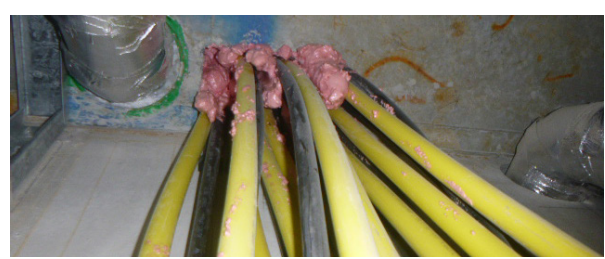
Traditional fire sealant and fire collar penetration systems need the fire walls to be installed first, and often compromise the deflection head of the wall (above). Multiple PEX pipes clustered into a small space is very difficult to provide a retrofit solution (below):
