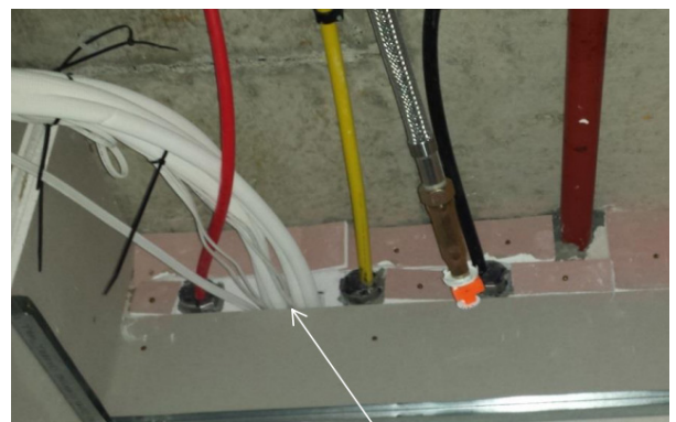
Traditional fire sealant and fire collar penetration systems need the fire walls to be installed first, and often compromise the deflection head of the wall (above). Multiple PEX pipes clustered into a small space is very difficult to provide a retrofit solution (below):
